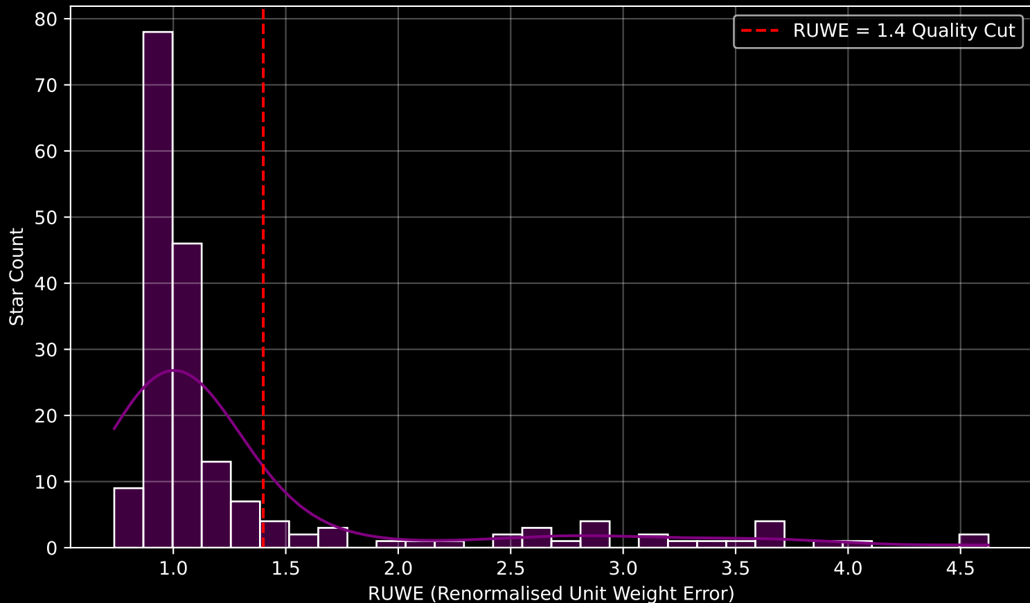
GAPOGEE DR17 Field [114+62_MGA] RUWE Distribution (n= 188)
