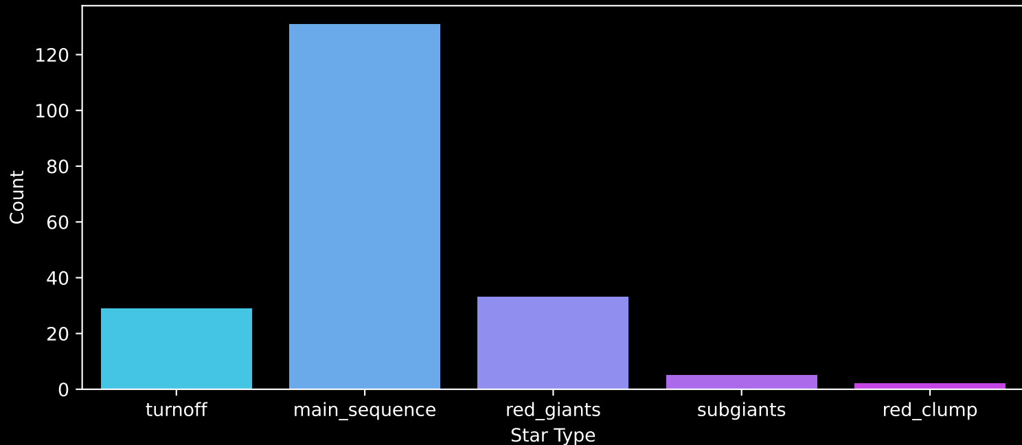
APOGEE DR17 Field: [114+62_MGA] Count plot of Star Type
