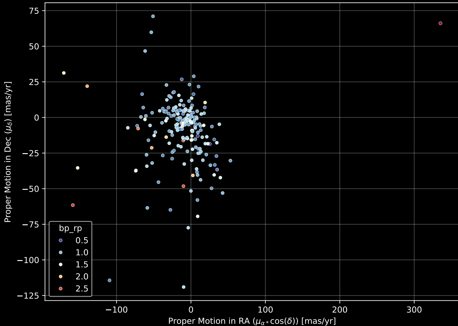
APOGEE DR17 Field: [114+62_MGA] Proper Motion Diagram (n= 200)
