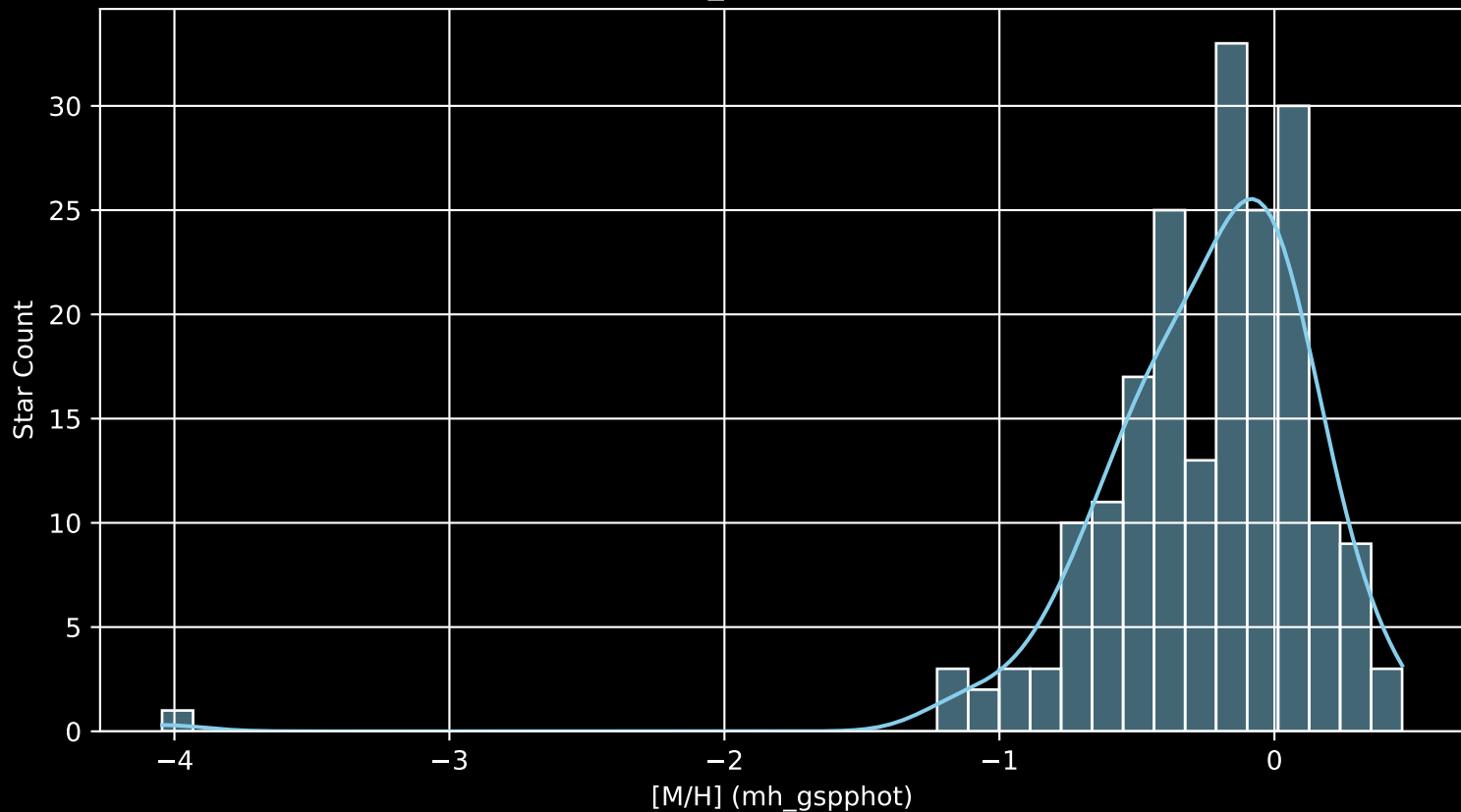
APOGEE DR17 Field: [114+62_MGA [M/H] (mh_gspphot) (n= 198)
