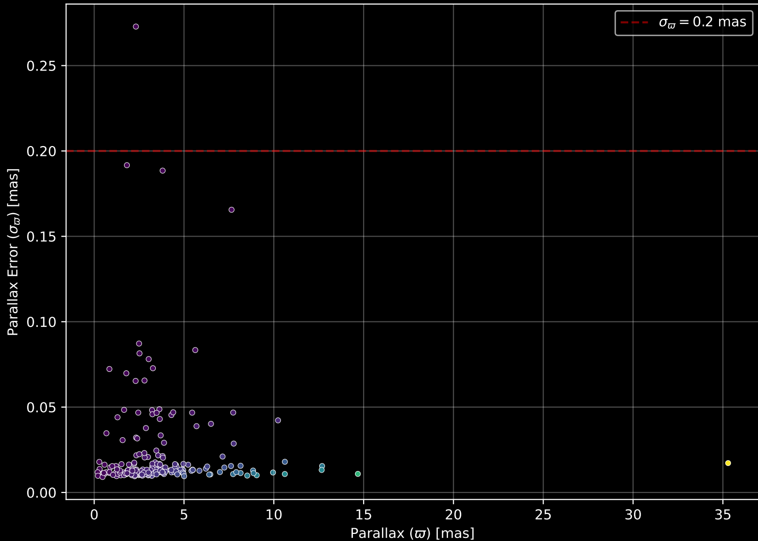
APOGEE DR17 Field: [114+62_MGA] Parallax Quality (n= 200)
